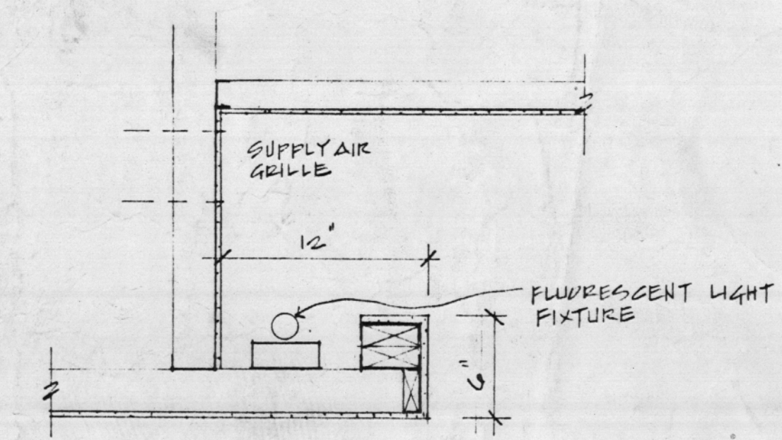
1 CEILING COVE DETAIL 1/2" = 1'-0"
