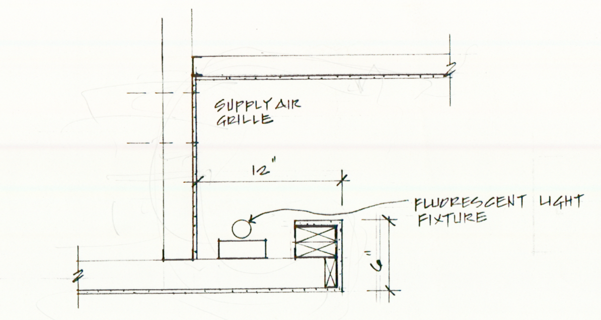
1 CEILING COVE DETAIL 5 1/2" = 1'-0"
