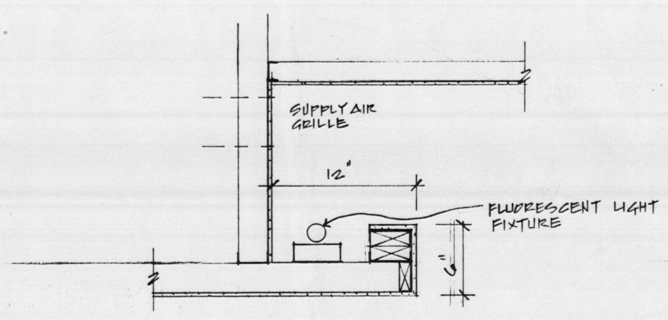
1 CEILING COVE DETAIL 5 1/2" = 1'-0"
