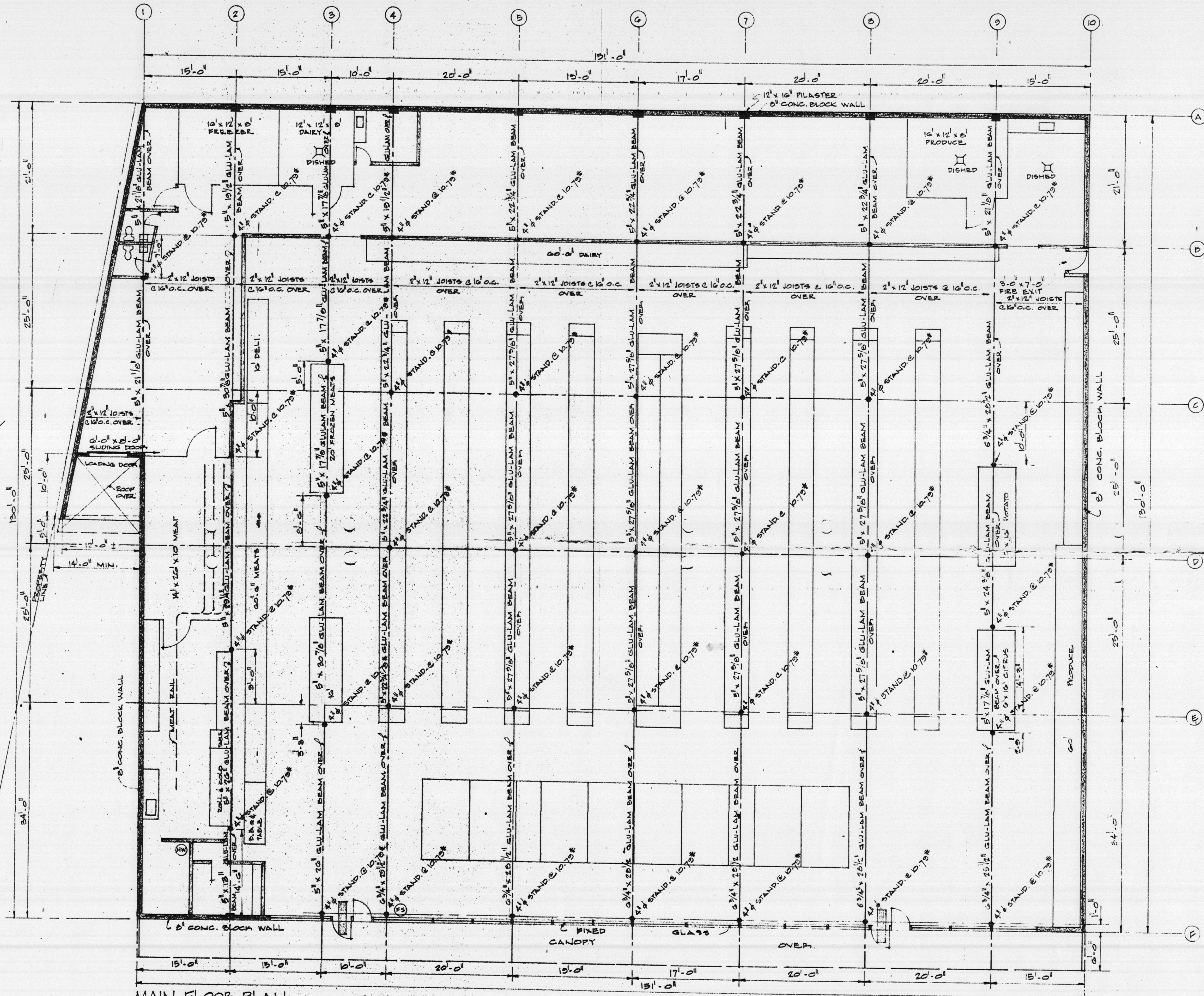
MAIN FLOOR PLAN SCALE 1/8" = 1'-0"
